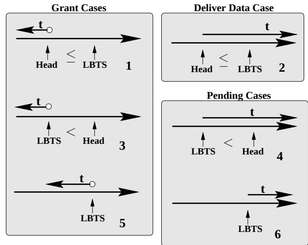
Figure 3: Time Stamp Order Event Queue Case Groupings
